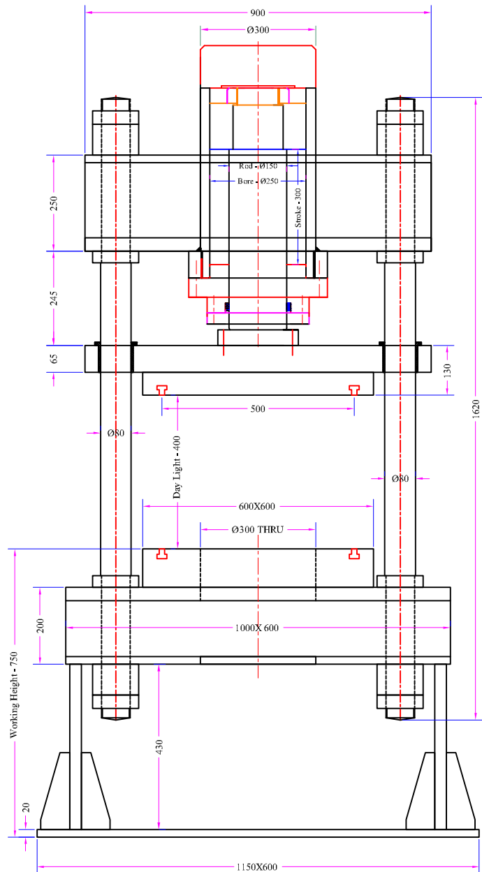
Front View
